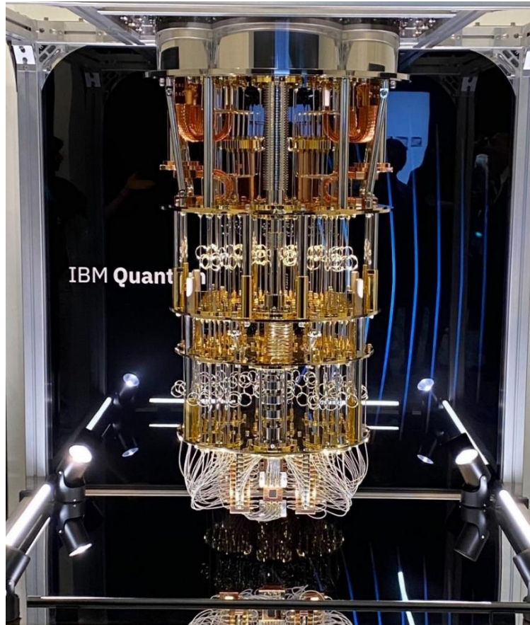
IBM Quantume System One 內部構造樣本展示
