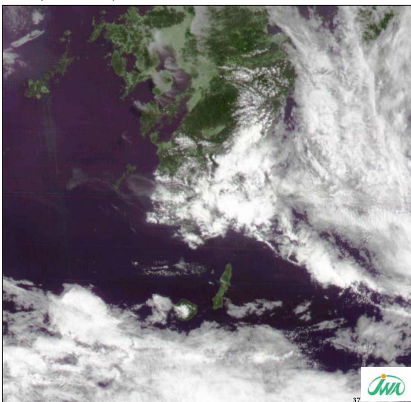
Sample-4 Eruption of Kuchierabu Is.
