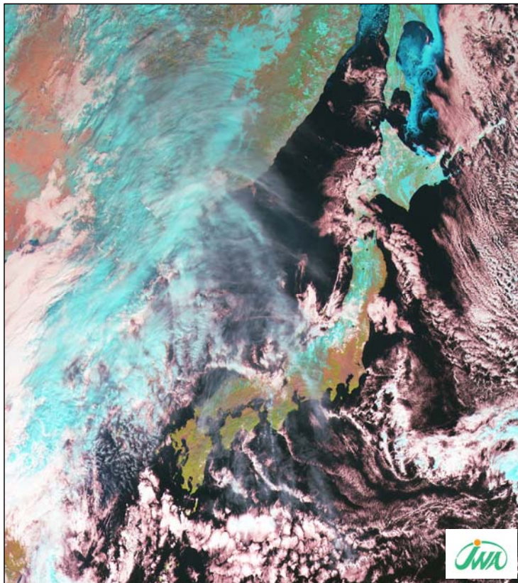
Sample-1 Natural Color RGB composite
