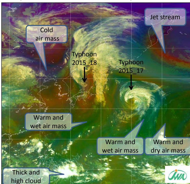
Sample-2 Airmass Color RGB composite
